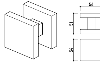
BASIC SIM - AISI 304
