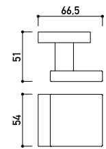
BASIC EXC - AISI 304
