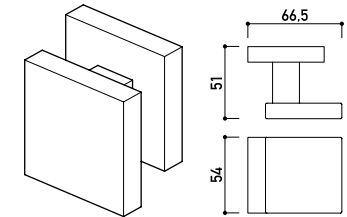
BASIC EXC - AISI 304
